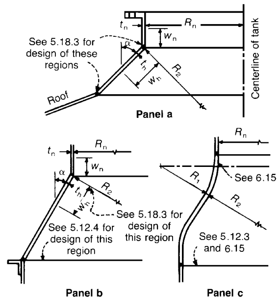
Figure 5-9—Large Head Openings and Conical Shell-Reducer Sections
