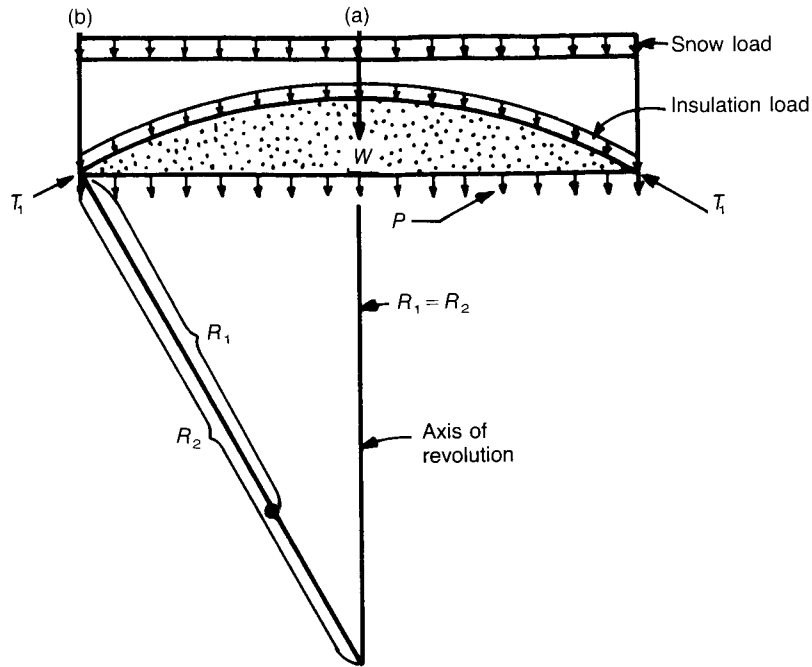
Figure F-4—Free-Body Sketch (See F.3)
