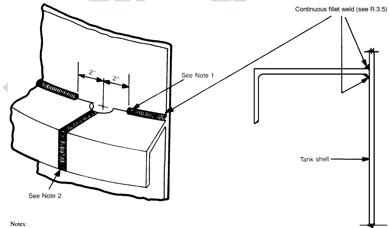
Figure R-1—Typical Stiffening-Ring Weld Details
