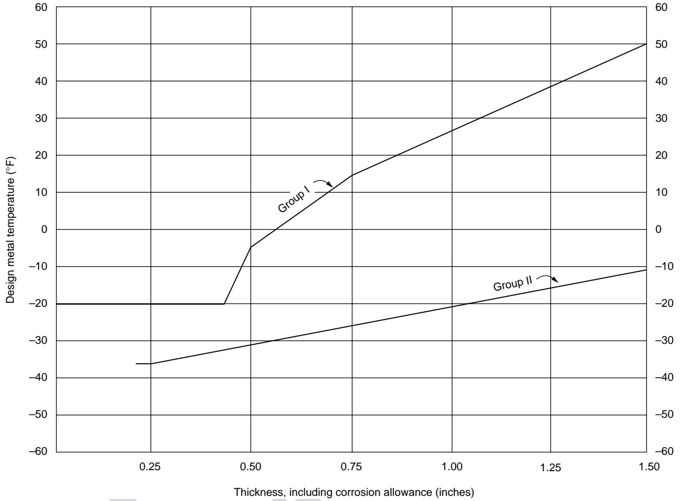
Figure 4-2—Minimum Permissible Design Metal Temperature for Pipe, Flanges, and Forgings without Impact Testing | 04
