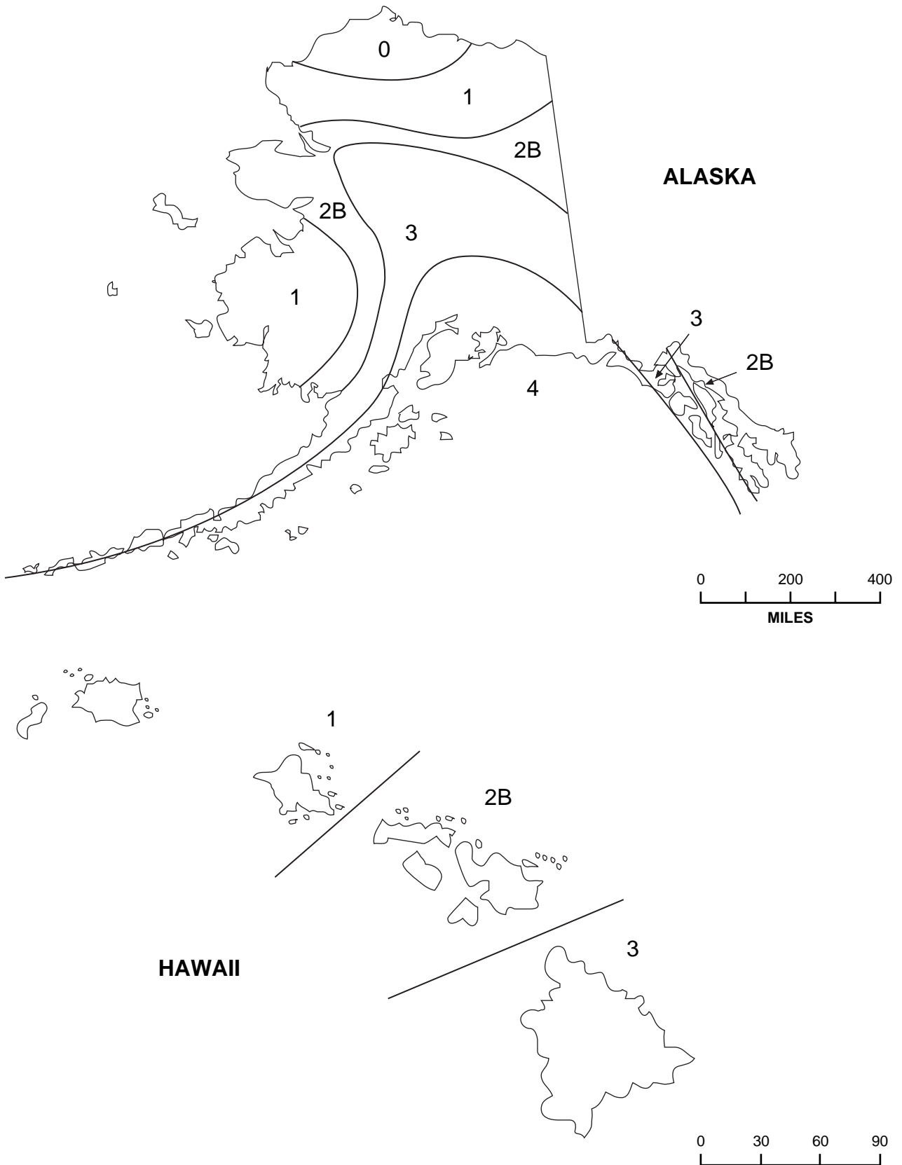
Figure L-1-Part 2—Seismic Zone Map
