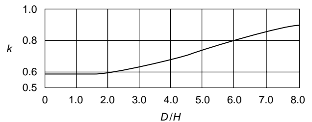
Figure L-4—Curve for Obtaining Factor k for the Ratio D/H
