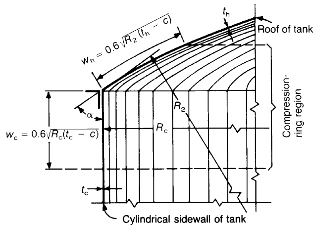
Figure 5-5—Compression-Ring Region
