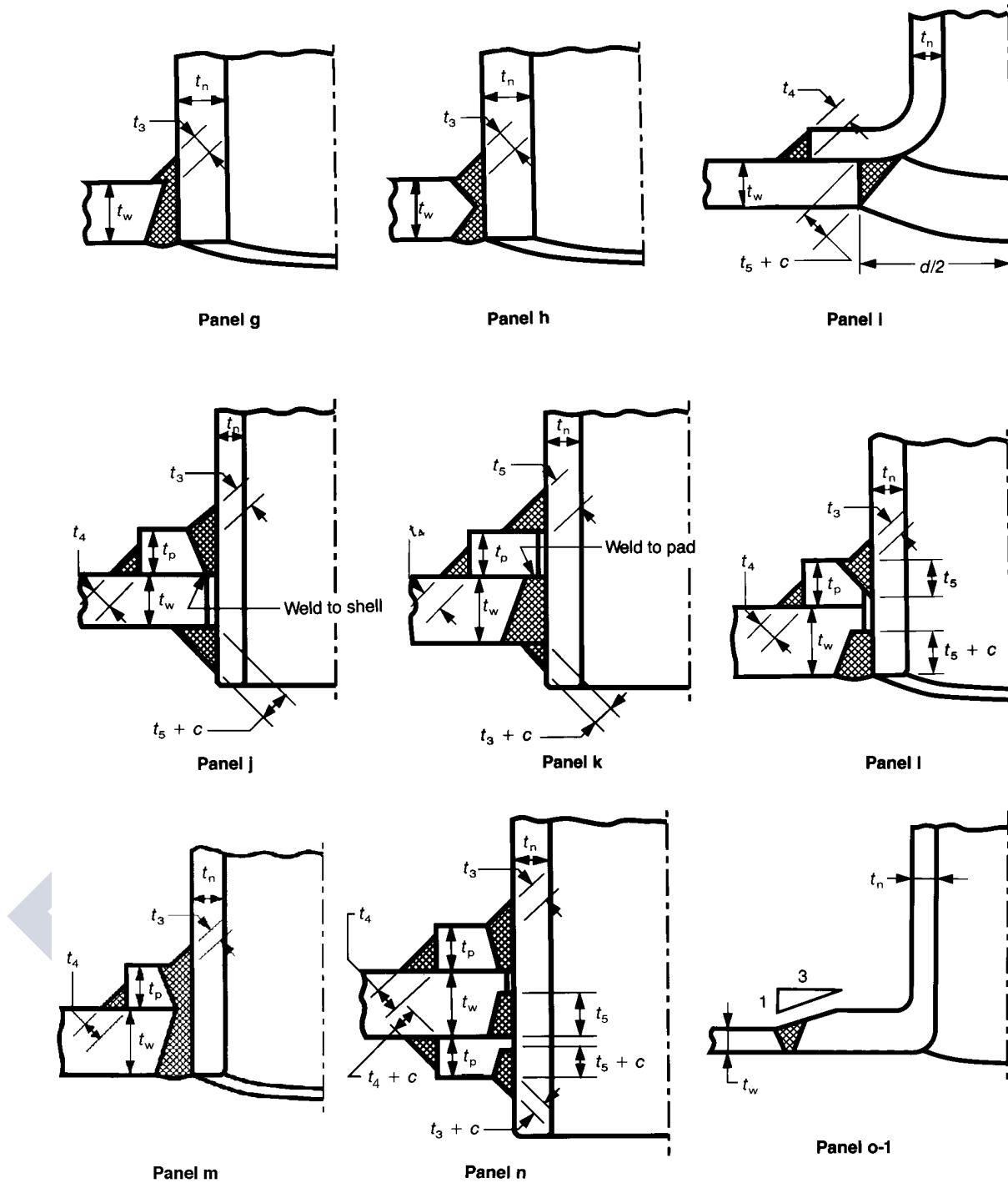
Figure 5-8-Part 2—Acceptable Types of Welded Nozzles and Other Connections
